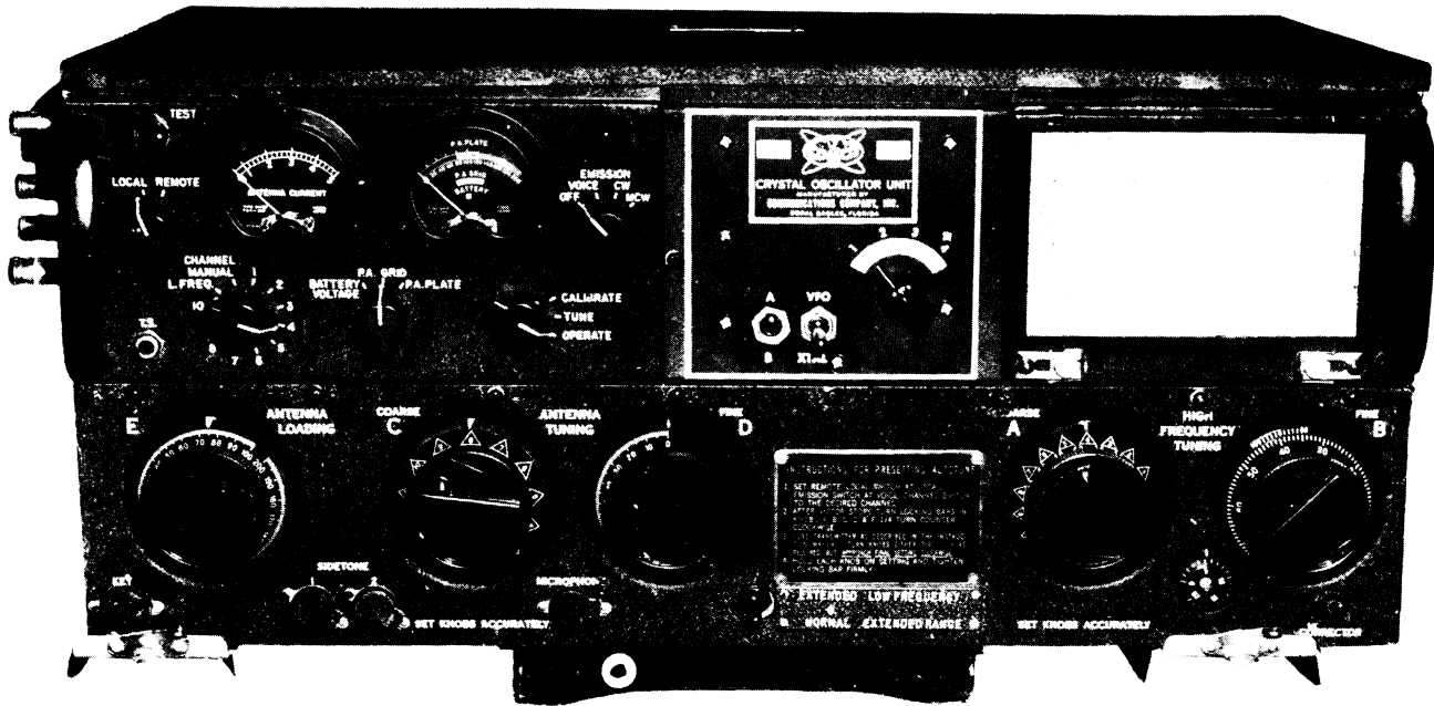
Figure 2-9 A. Radio Transmitter T-4 12/ART-13B — Front View
