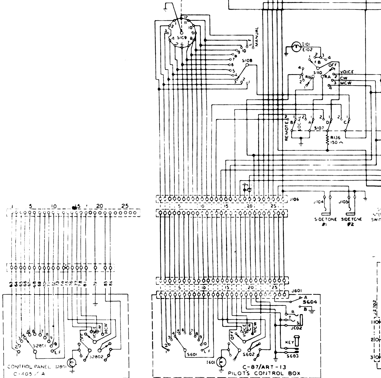
ALTERMAFF TO PILOT'S CONTROL BOX C-87/ART-13
